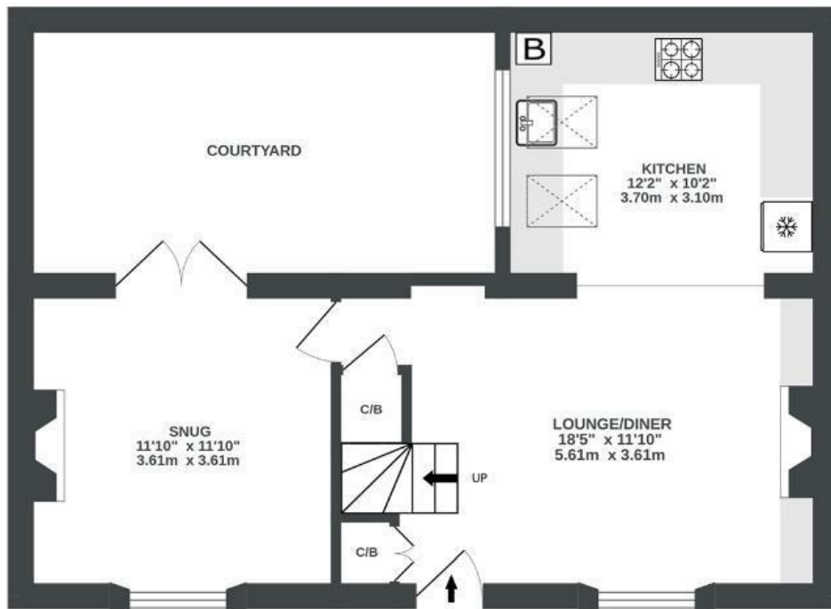
GROUND FLOOR 482 sq.ft. (44.8 sq.m.) approx.
